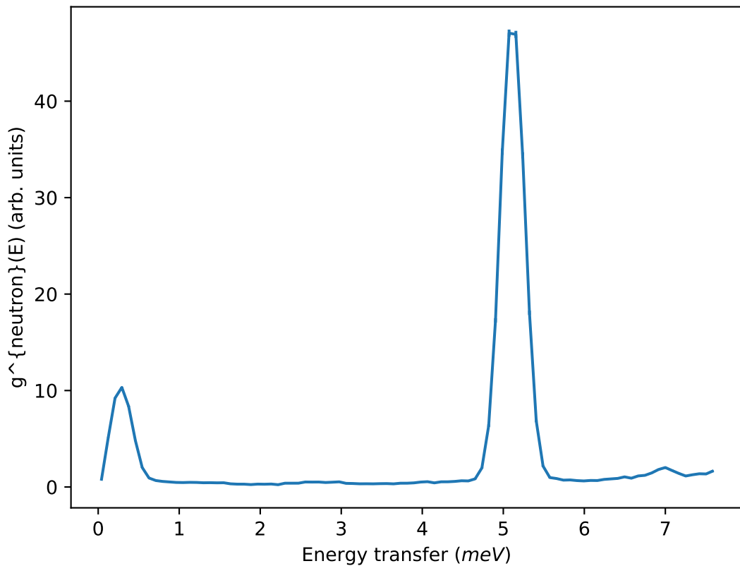
Density of states from S(2\theta, W)
