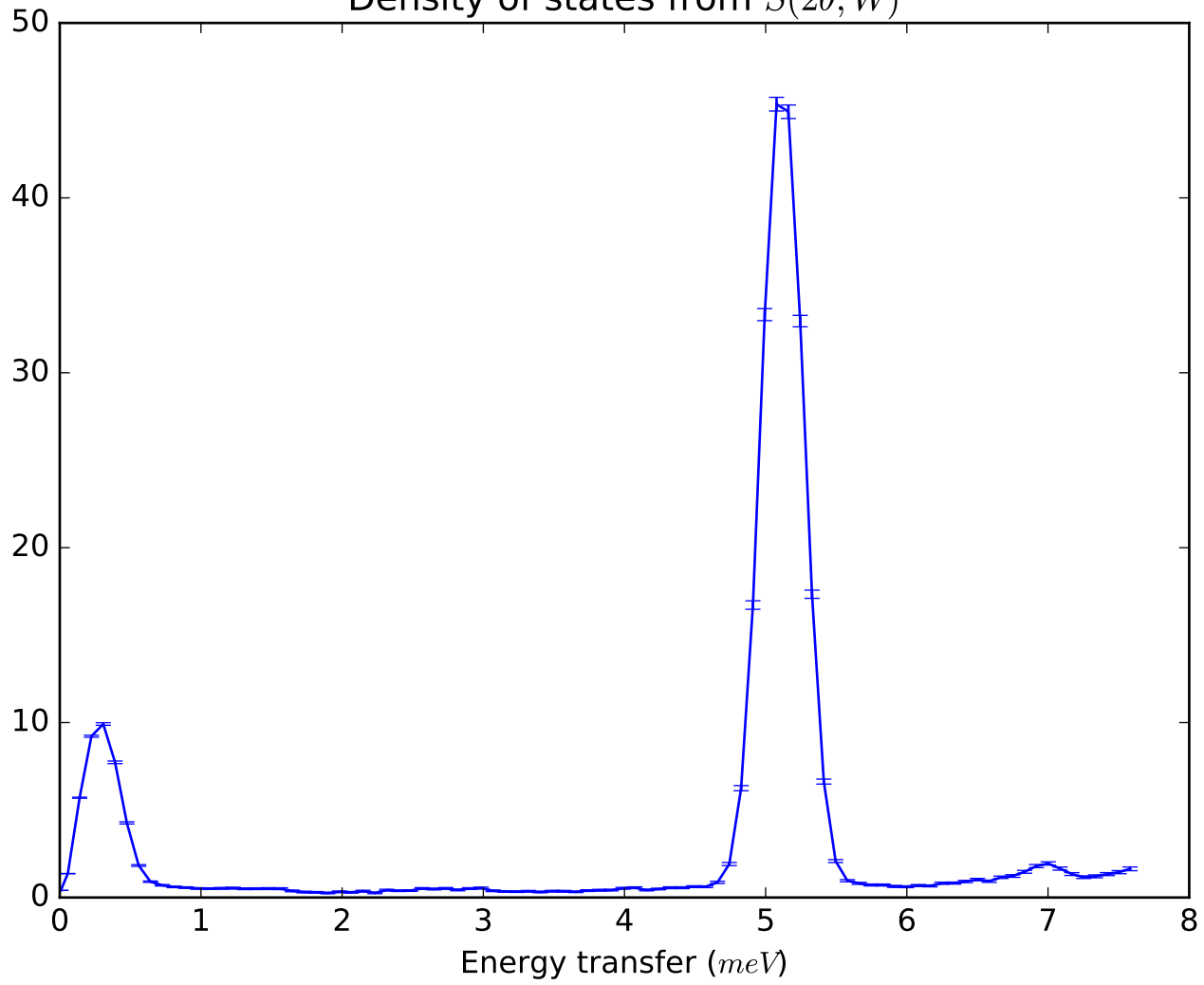
Density of states from S(2\theta, W)
