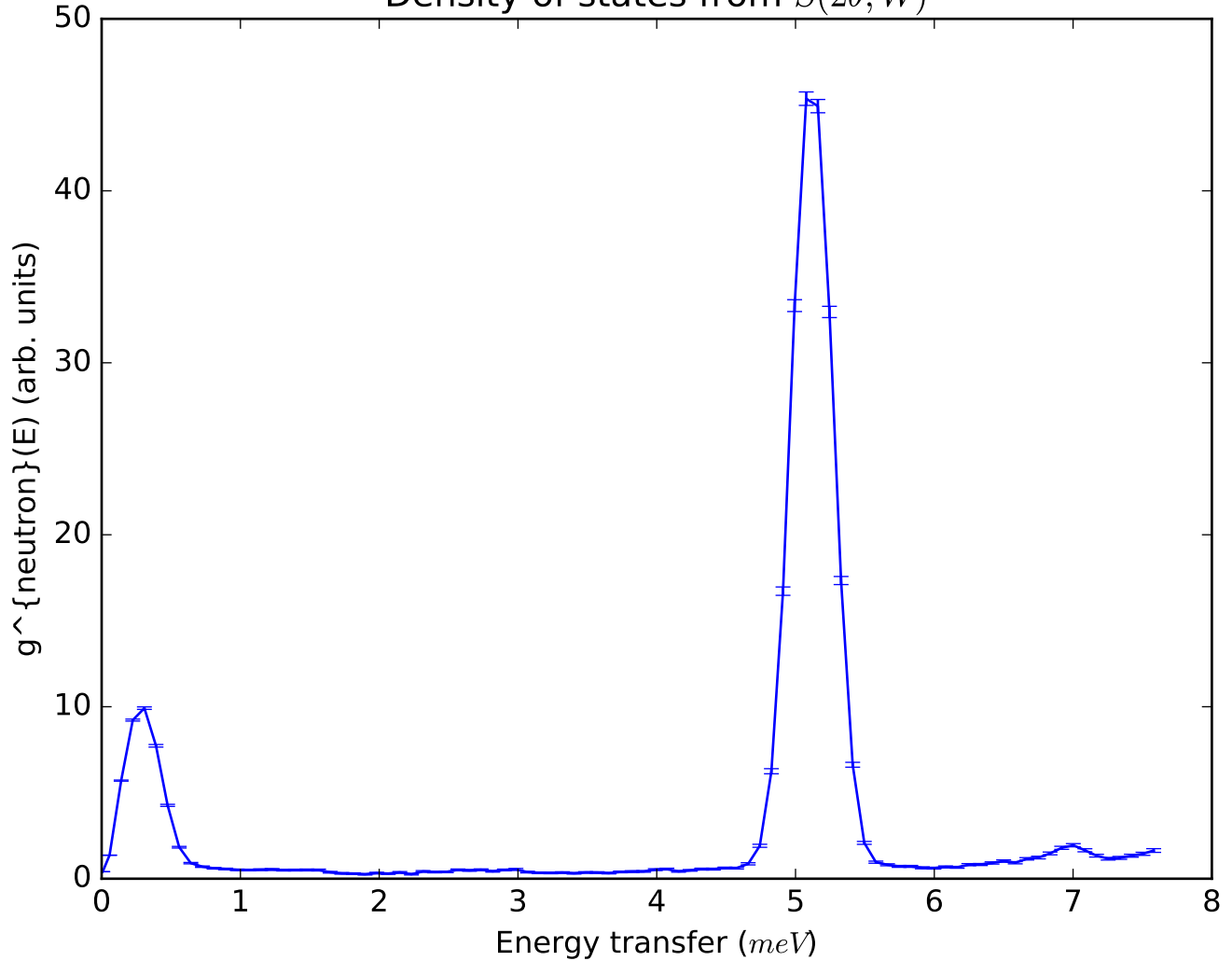
Density of states from S(2\theta, W)
