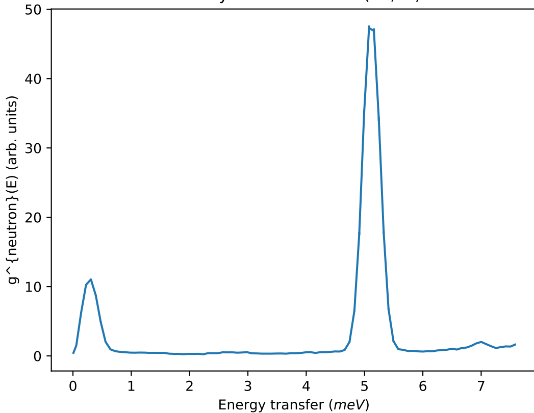
Density of states from S(2\theta, W)
